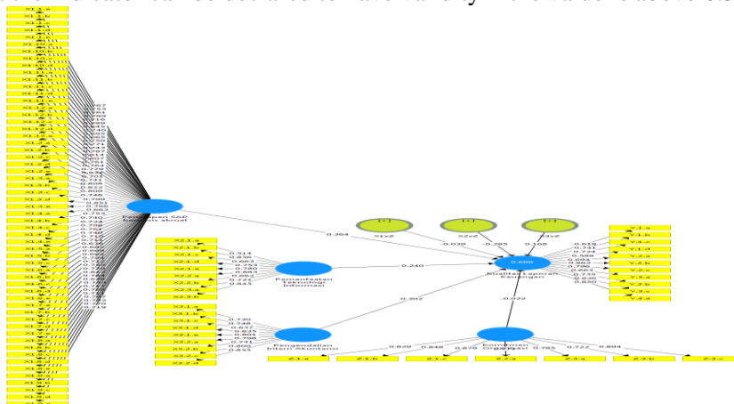
Figure 1 PLS Model
